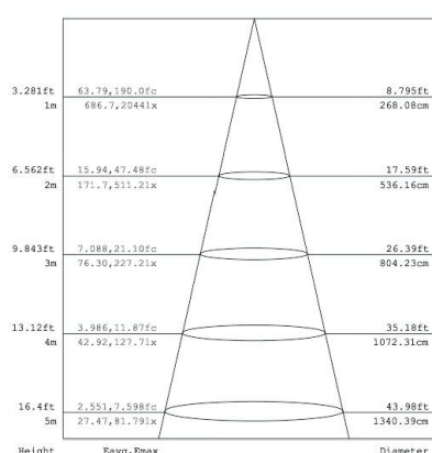
Cone Illuminance Diagram:
