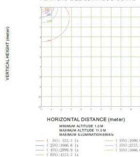
VERTICAL EQUILUMINOUS CURVE
