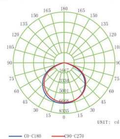
HY-UFO-150W-110-H-3W3CCT LUMINOUS INTENSITY DISTRIBUTION DIAGRAM
