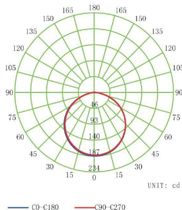
9W 4" Round LED Ultra Slim Downlight LUMINOUS INTENSITY DISTRIBUTION DIAGRAM
