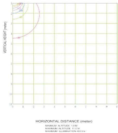
VERTICAL EQUILUMINOUS CURVE
